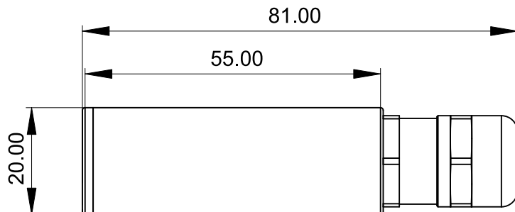
Microphone Capsule without Protection
