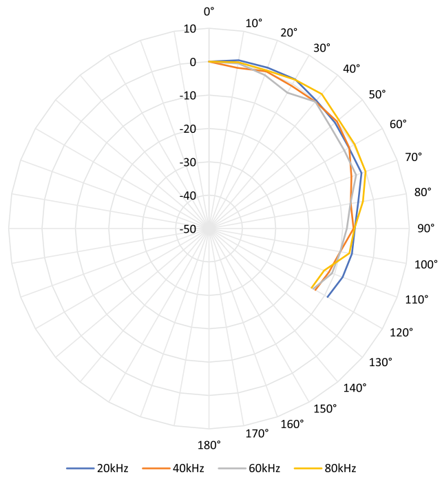
Directivity TM20S (without Microphone Capsule Protection)
