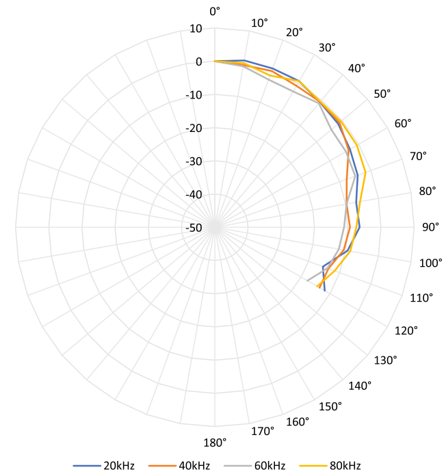
Directivity TM20S+ (with water repellant Microphone Capsule Protection)
